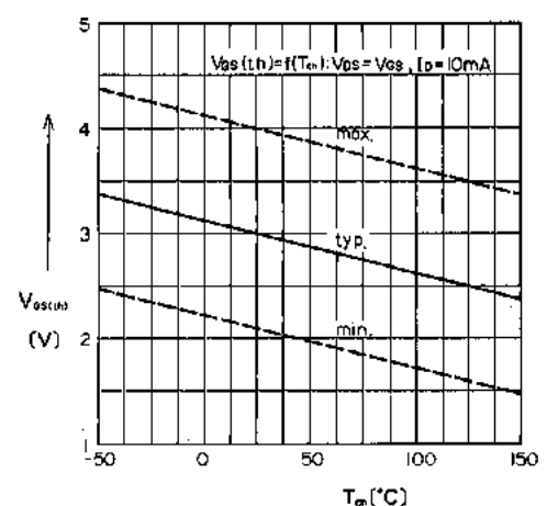
Gate Threshold Voltage vs T_m
