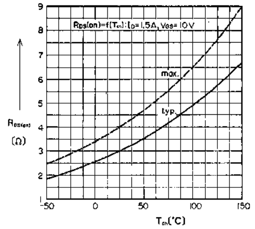
On State Resistance vs. T_m
