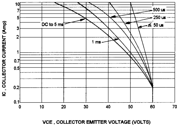
2N3789,2N3791
