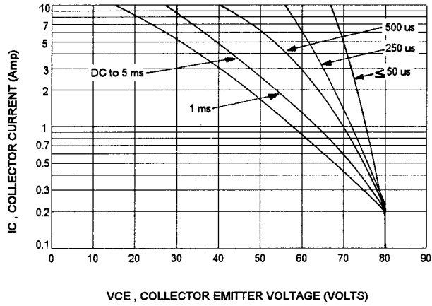
2N3790,2N3792
