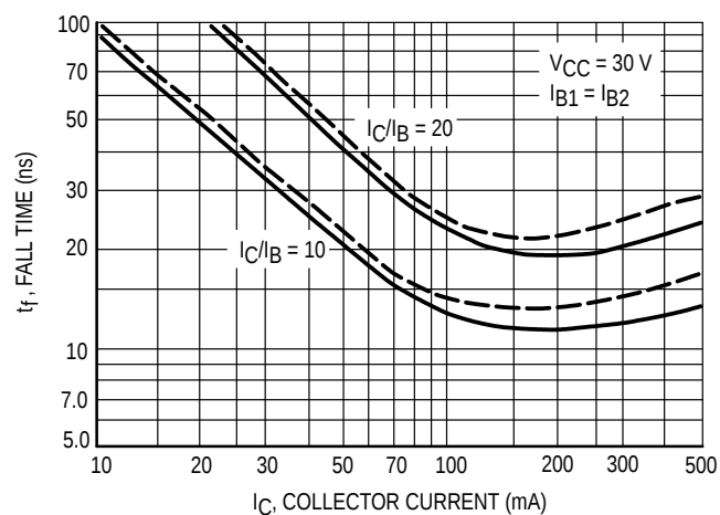
Figure 8. Fall Time
