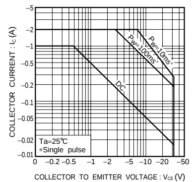
Fig.9 Safe operation area (2SB1132)
