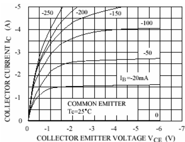
Fig.3 Static Characteristic
