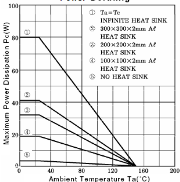
Power Derating
