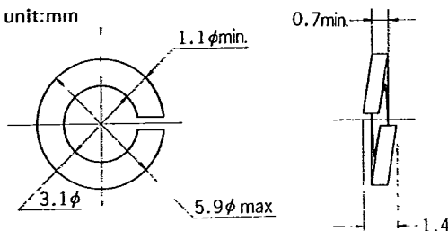
Case Outline—[0015]
