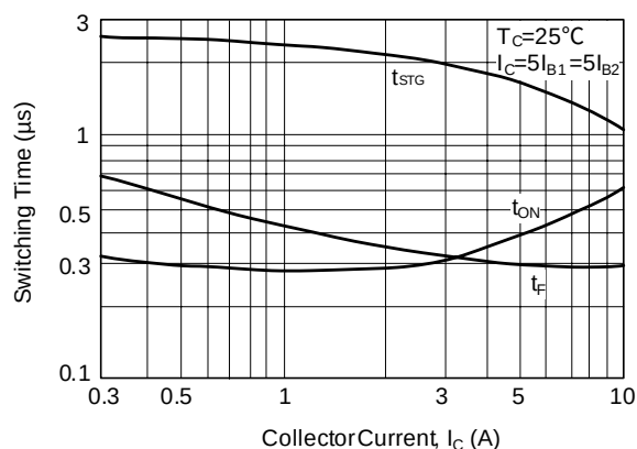
Switching Time
