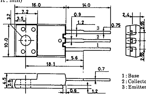
Package Dimensions 2079A (unit: mm)
