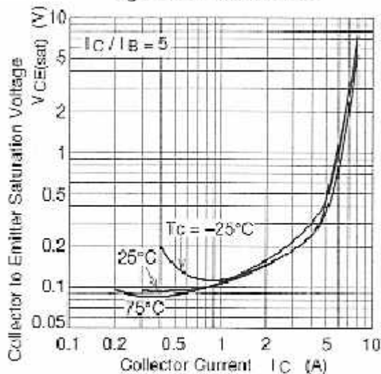
Fig.5 Collector-Emitter Saturation Voltage
