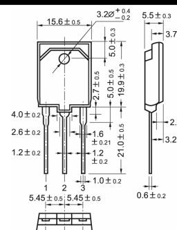
TO-3PFM
