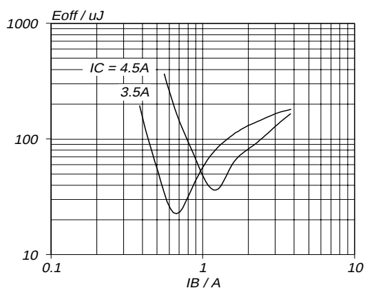
Fig.11. Typical turn-off losses. T_J = 85^\circ\text{C} E_{off} = f(I_B) ; parameter I_C
