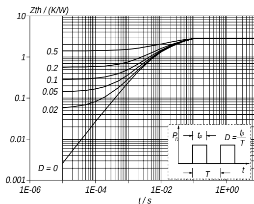
Fig.16. Transient thermal impedance. Z_{th\text{-}j\text{-}hs} = f(t) ; parameter D = t_p / T
