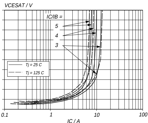
Fig.6. Typical collector-emitter saturation voltage. V_{CEsat} = f(I_C) ; parameter I_C/I_B
