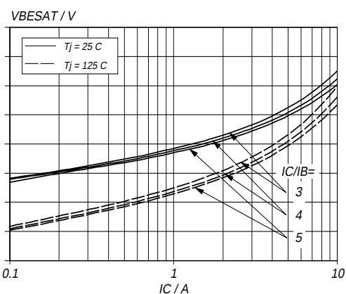
Fig.5. Typical base-emitter saturation voltage. V_{BE\text{sat}} = f(I_C) ; parameter I_C/I_B
