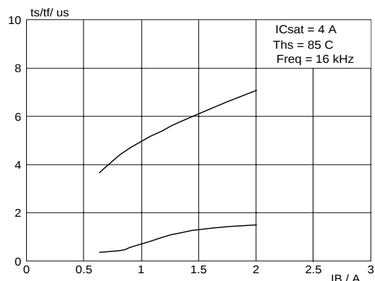
Fig.9. Typical collector storage and fall time. I_{C\ sat} = 4\ A; T_j = 85^\circ C; f = 16\ kHz
