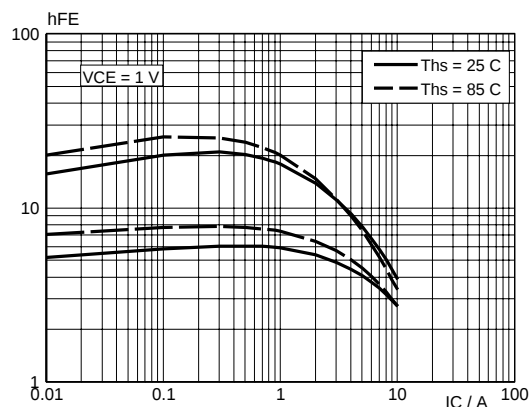
Fig. 7. High and low DC current gain.
