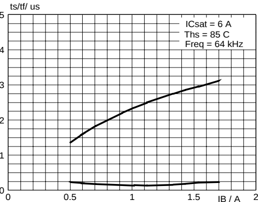
Fig. 12. Typical collector storage and fall time. I_C = 6\text{ A} ; T_j = 85^\circ\text{C} ; f = 64\text{ kHz}
