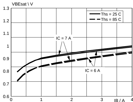
Fig. 10. Typical base-emitter saturation voltage.
