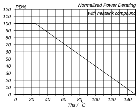
Fig.13. Normalised power dissipation. PD\% = 100 \cdot P_D / P_{D\ 25^\circ C}
