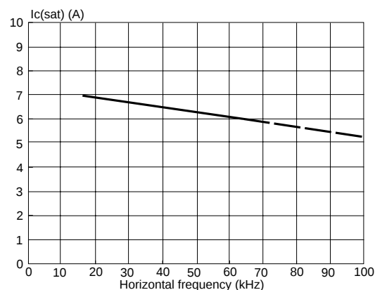
Fig.17. I_{Csat} during normal running vs. frequency of operation for optimum performance
