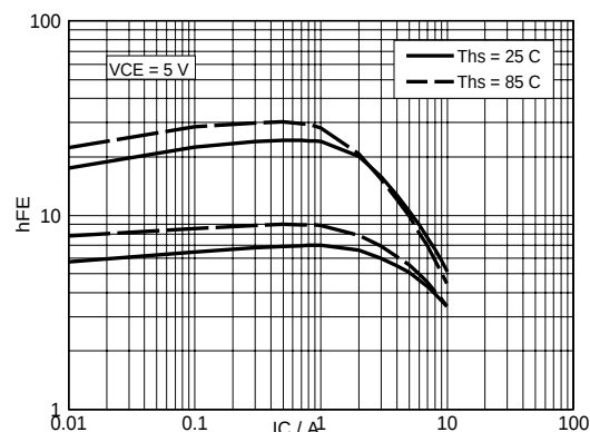
Fig. 8. High and low DC current gain.
