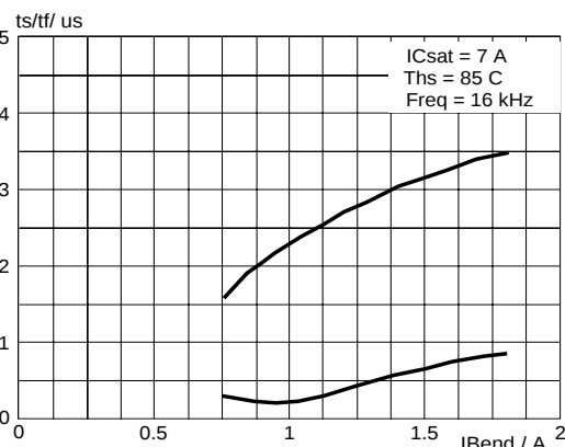
Fig. 11. Typical collector storage and fall time. I_C = 7\text{ A} ; T_j = 85^\circ\text{C} ; f = 16\text{ kHz}
