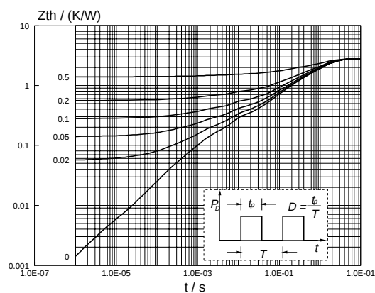
Fig.14. Transient thermal impedance.
