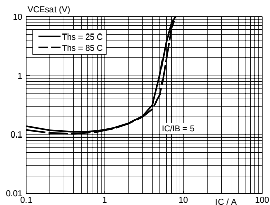
Fig. 9. Typical collector-emitter saturation voltage.
