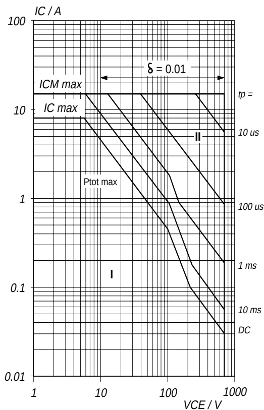
Fig.12. Forward bias safe operating area. T_{hs} = 25^{\circ}\text{C}
