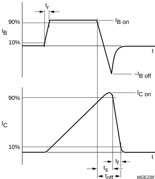
Fig.14 Switching times waveforms with inductive load.
