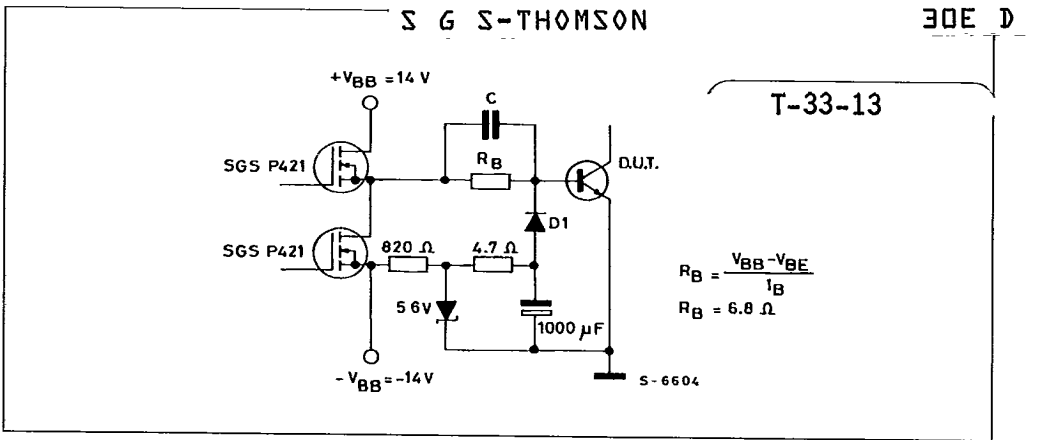
Figure 5 : Equivalent Input Schematic Circuit at Turn-on.
