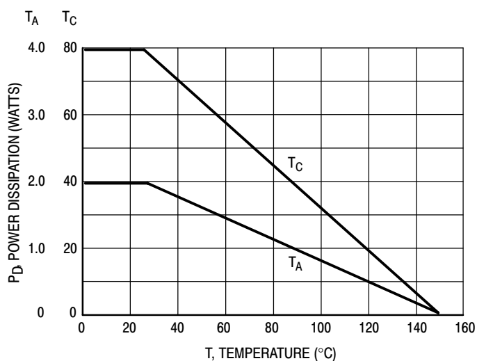
Figure 1. Power Derating
