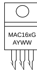
TO-220AB CASE 221A-09 STYLE 4
