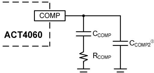
Figure 2: Stability Compensation
