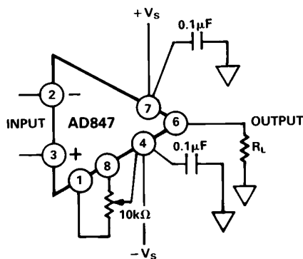
Figure 21. Offset Nulling
