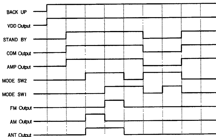
Figure 5 Timing chart
