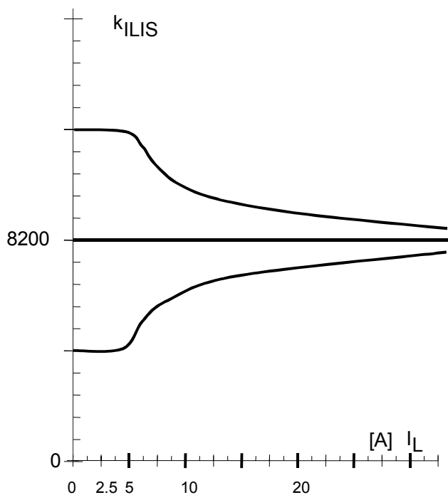
Figure 6b: Current sense ratio 12) :
