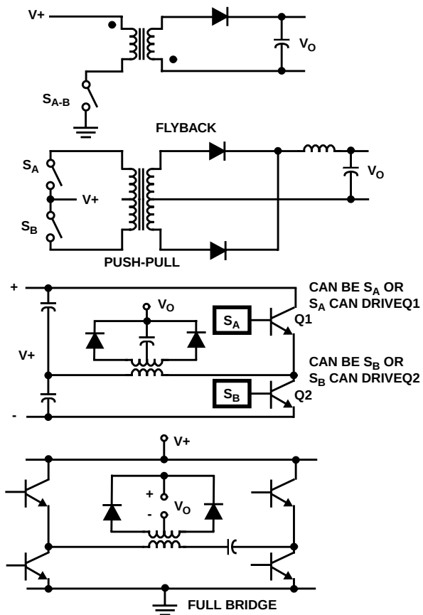
FIGURE 17. TRANSFORMER-COUPLED OUTPUTS
