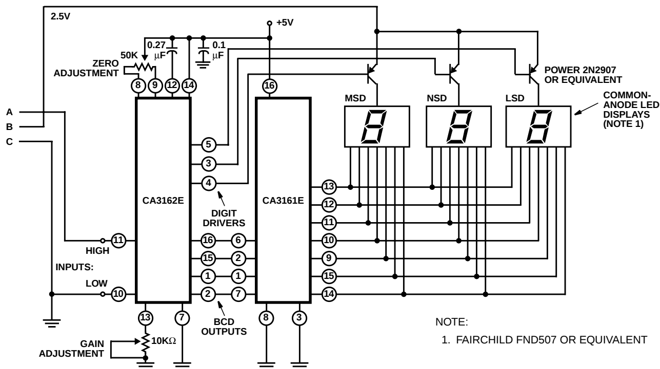
FIGURE 25. SCHEMATIC DIAGRAM OF DIGITAL READOUT SCALE (CONT'D)
