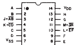
CD4011B
