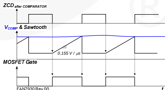
Figure 32. Turn-On Time Determination
