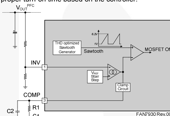
Figure 31. Control Circuit
