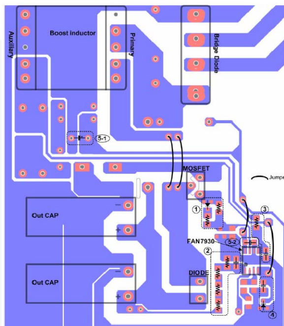
Figure 43. Recommended PCB Layout
