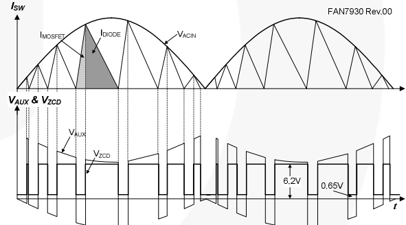
Figure 27. Auxiliary Voltage Depends on MOSFET Switching
