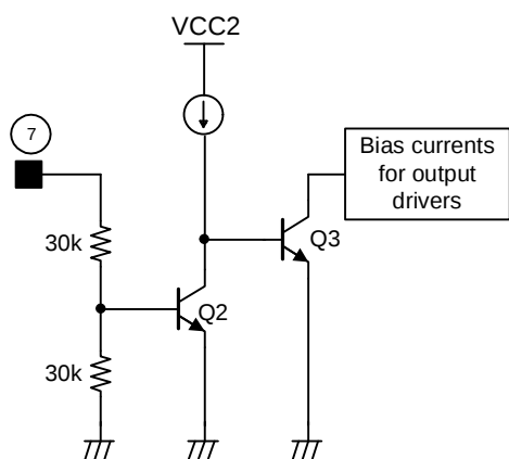
Fig. 2. All mute function using the MUTE pin
