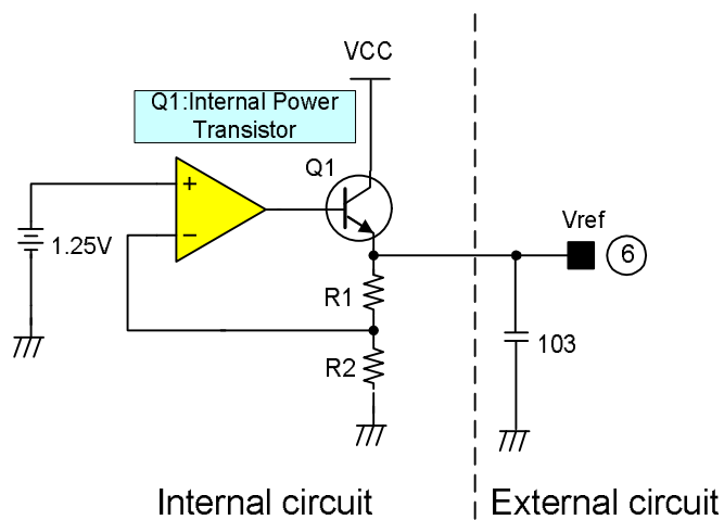
Fig. 4. Regulator
